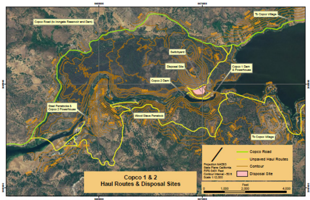
Figure 4.2-2 – Proposed Haul Routes and Disposal Sites for Copco No. 1 Dam.
