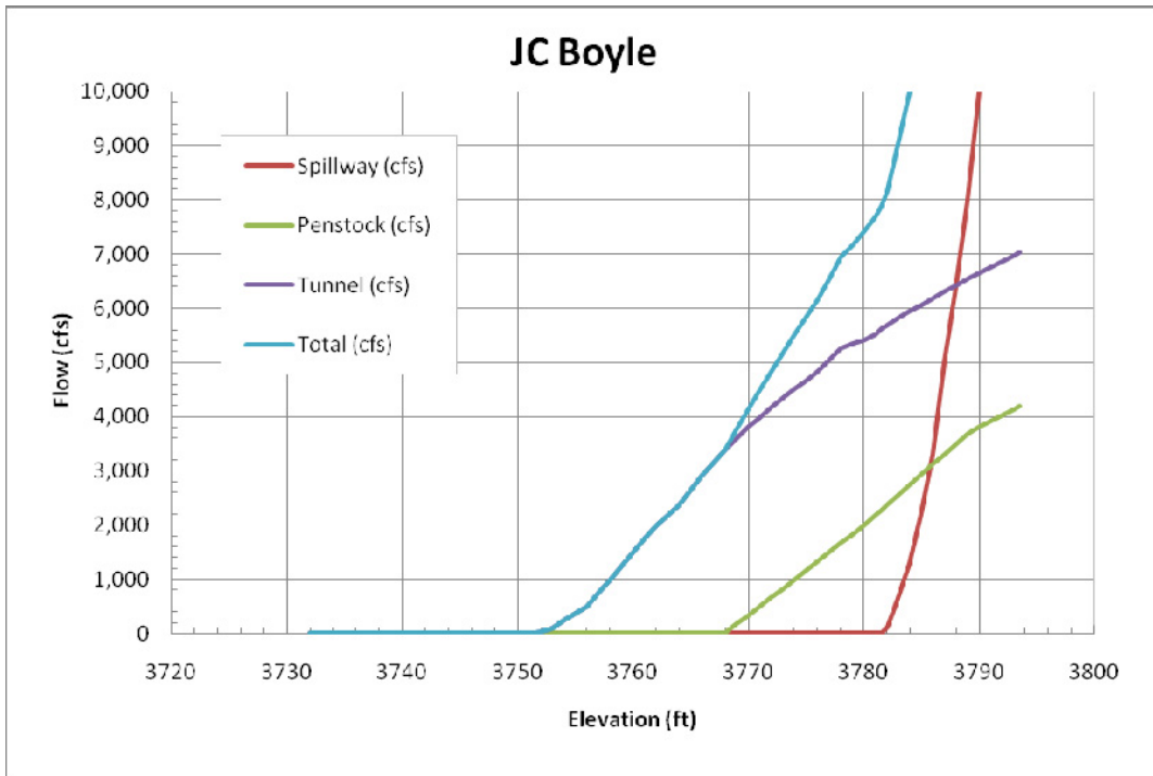
Figure 5.11. Outlet Capacities at J.C. Boyle.
