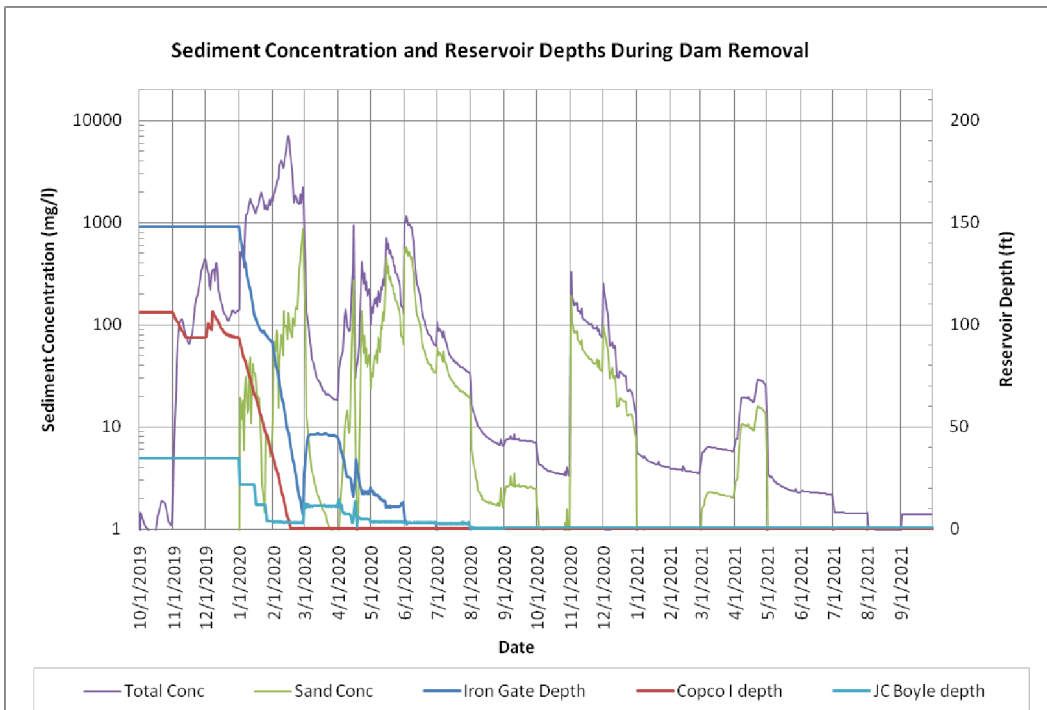
Figure 5.16. Reservoir depth and sediment concentrations downstream of Iron Gate Dam during drawdown for a wet year.
