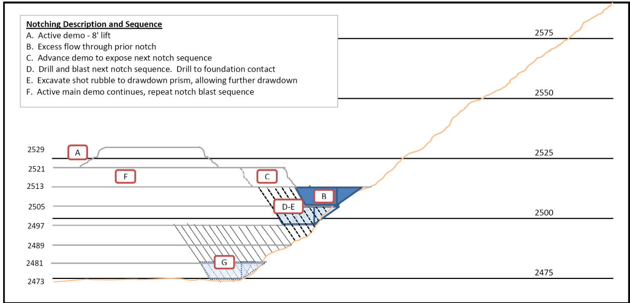
Figure 4.2-1 – Proposed Notching Sequence for Copco No. 1 Dam.
