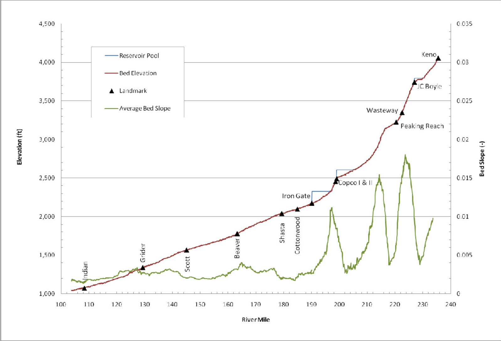
Figure 5.12. Bed Elevation Profile in Reach from Keno to Happy Camp.
