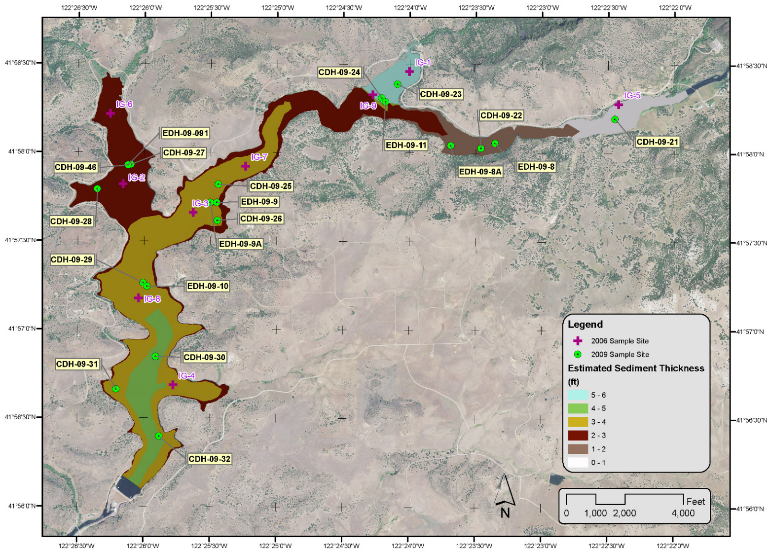
Figure 5.7. Iron Gate Estimated Sediment Thickness and Sample Site Locations.
