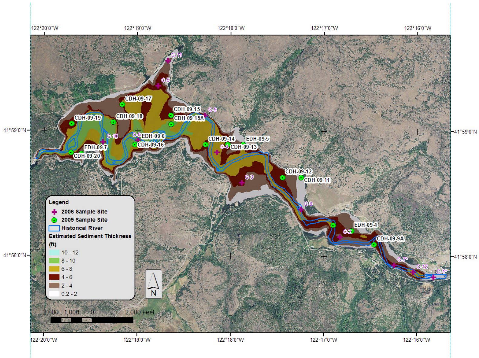
Figure 5.6. Copco 1 Estimated Sediment Thickness and Sample Site Locations.
