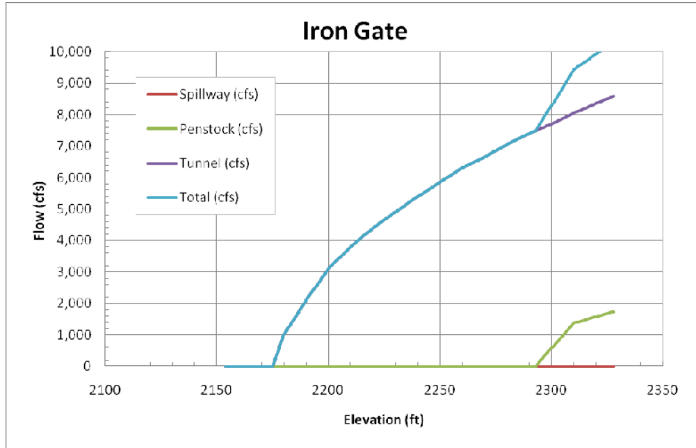
Figure 5.9. Outlet Capacities at Iron Gate.
