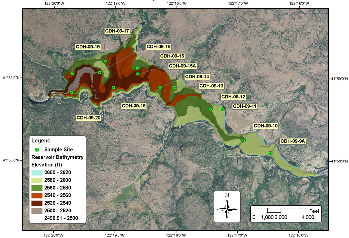
Figure 5.2. Bathymetry of Copco 1 and 2009 Drill Hole Locations.
