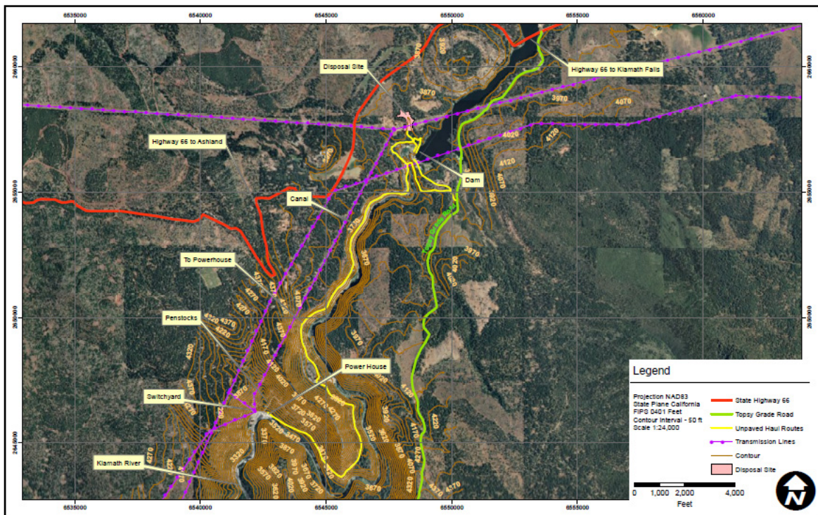
Figure 4.1-1. – Proposed Haul Routes and Disposal Sites for J.C. Boyle Dam.
