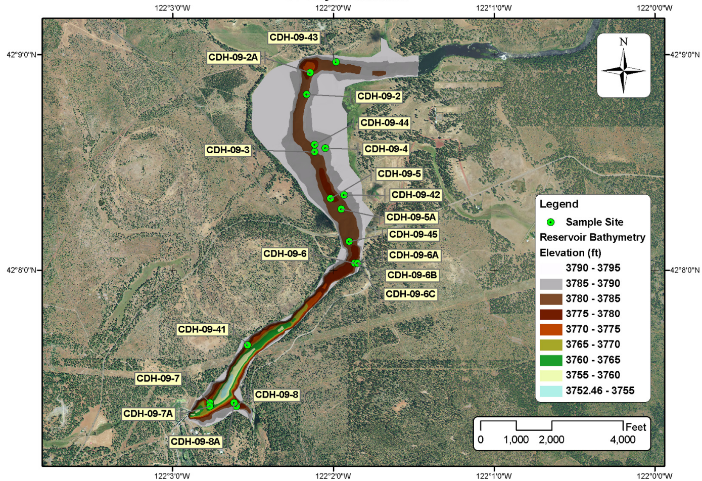
Figure 5.1. Bathymetry of JC Boyle and 2009 Drill Hole Locations.
