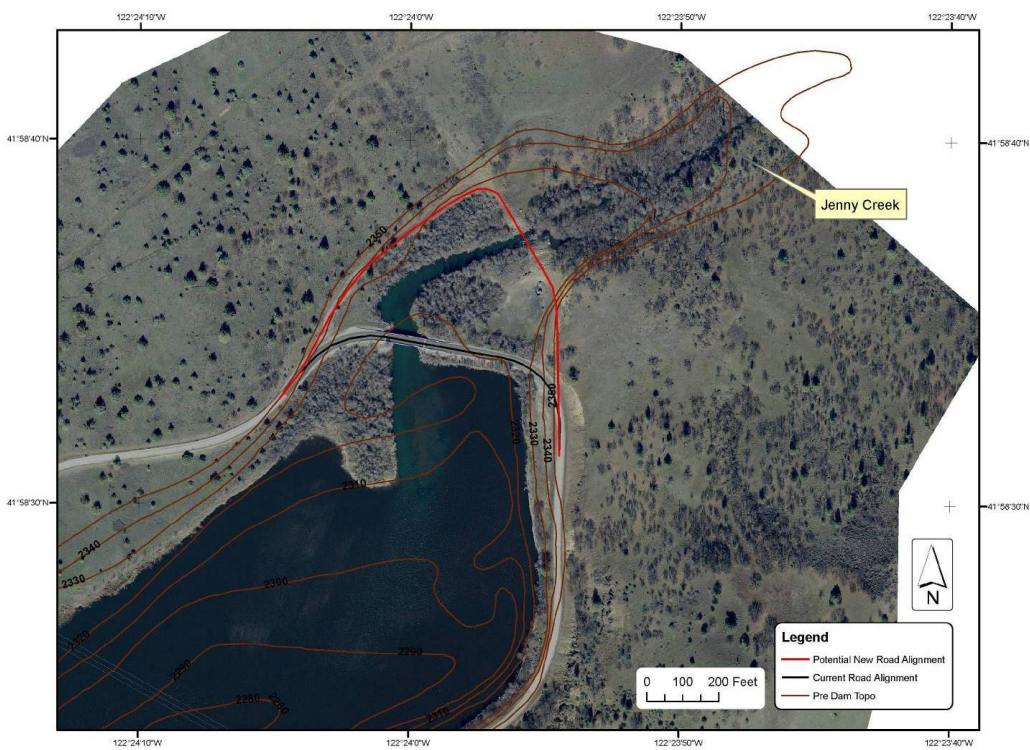
Figure 9.7-1. Location of Jenny Creek Bridge on delta deposits.
