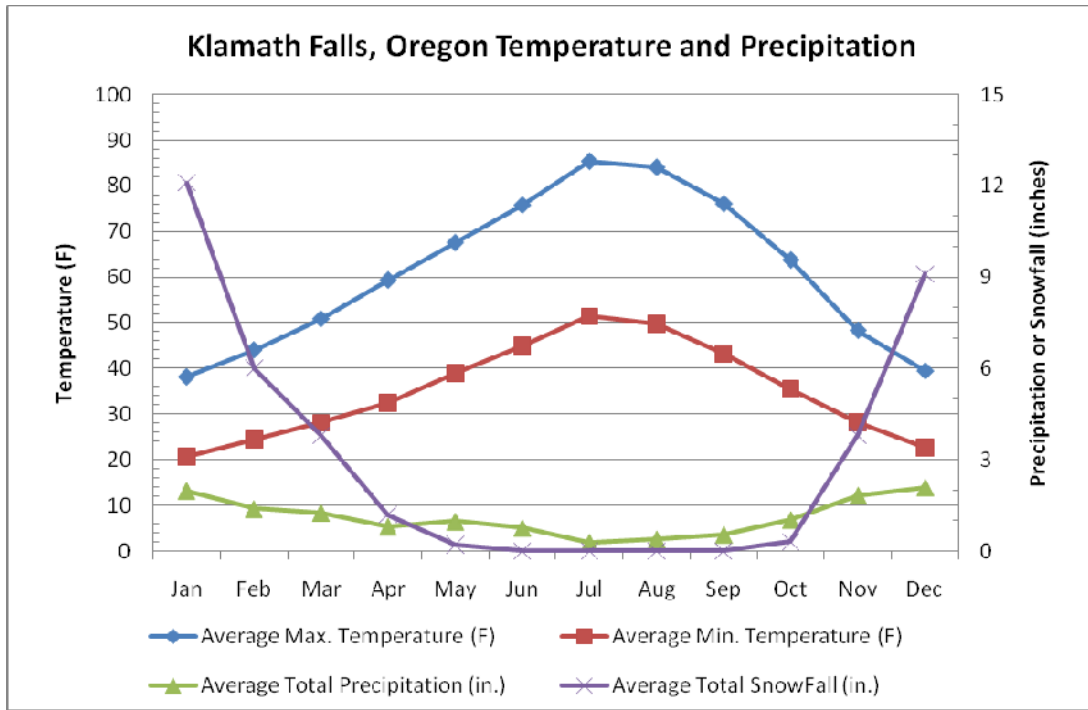
Figure 3.1. Average monthly temperatures and precipitation at Klamath Falls. (gage # 354506 at 41.97972 N, 122.33778 W). Period of record is from 5/11/1887 to 5/31/2001. Data obtained from Western Regional Climate Center ( http://www.wrcc.dri.edu/ ).
