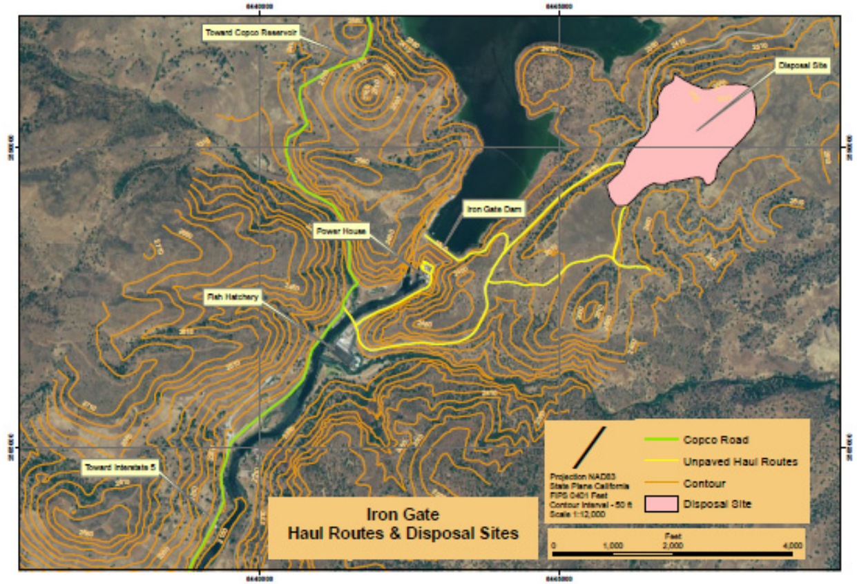
Figure 4.4-1. – Proposed Haul Routes and Disposal Sites for Iron Gate Dam.
