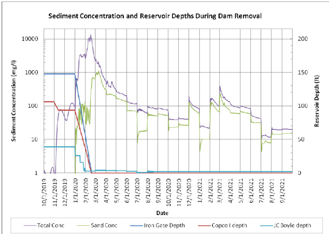
Figure 5.14. Reservoir depth and sediment concentrations downstream of Iron Gate Dam during drawdown for a dry year.
