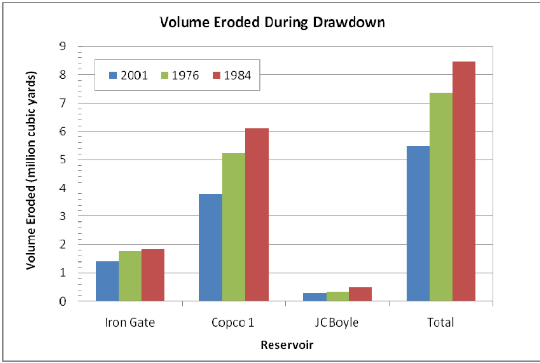
Figure 5-13. Volume of sediment erosion for preferred drawdown scenario.
