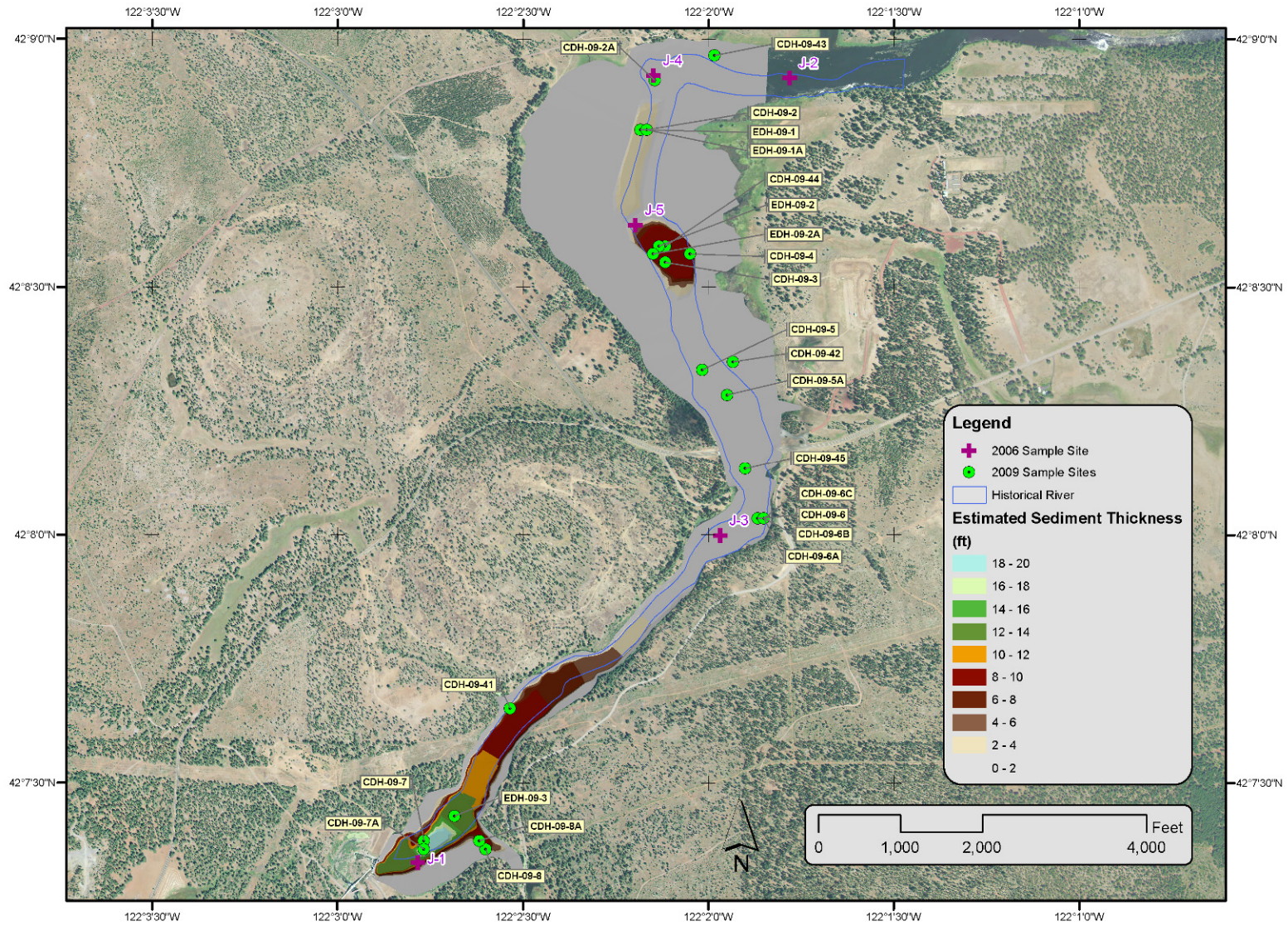
Figure 5.5. J.C. Boyle Estimated Sediment Thickness and Sample Site Locations.
