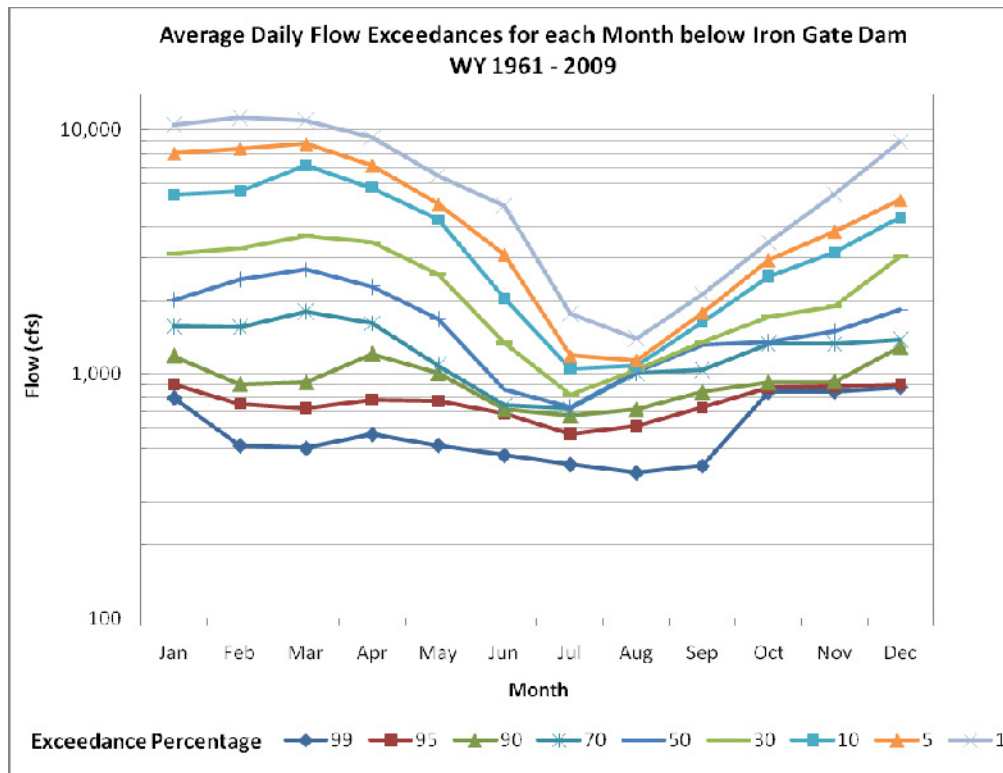
Figure 3.5. Daily average flow statistics for each month on the Klamath River at Iron Gate gage for the period of record WY 1961 – 2009.
