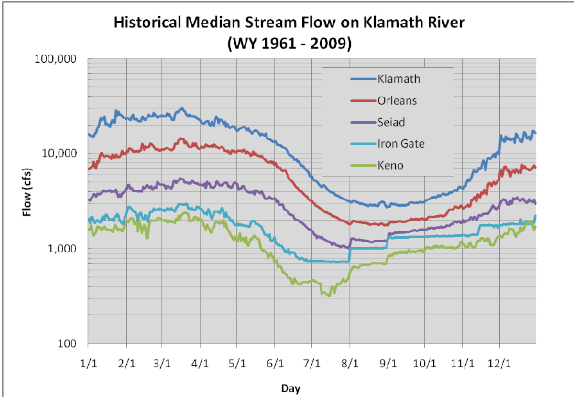
Figure 3.3. Median Flows at USGS stream gages on Klamath River.
