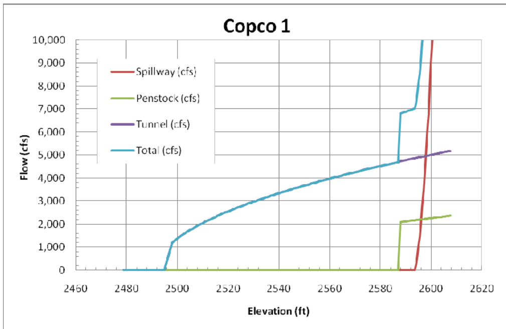
Figure 5.10. Outlet Capacities at Copco 1.
