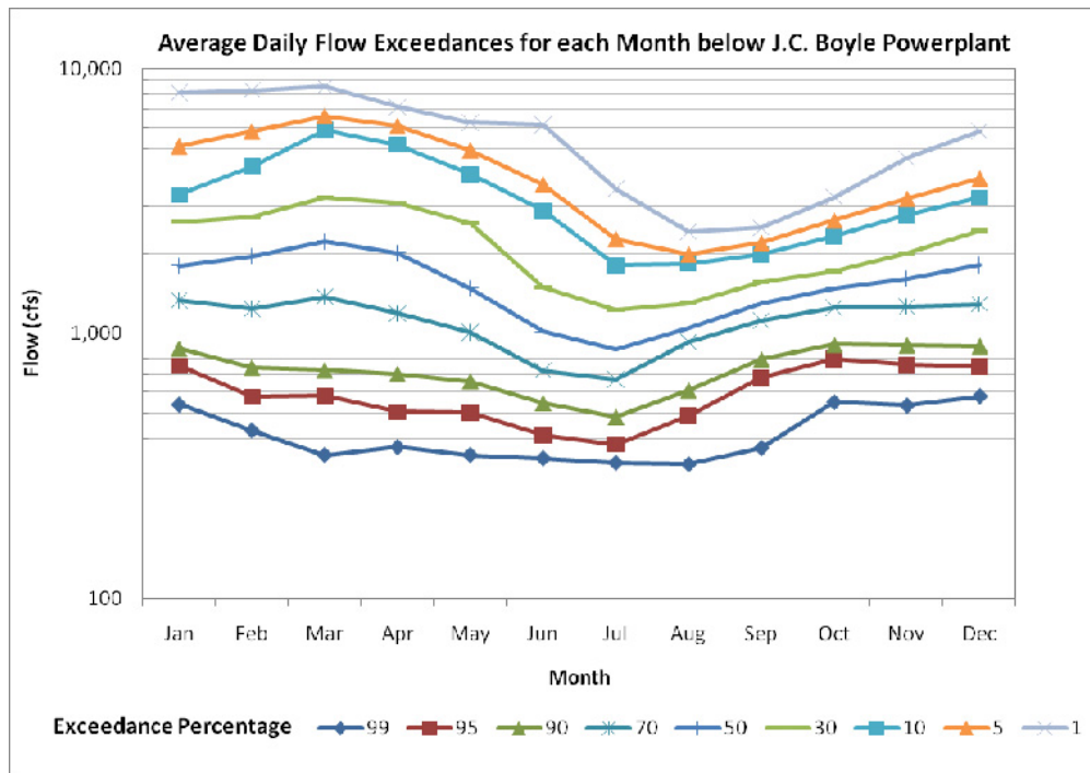
Figure 3.4. Stream Flow Statistics for JC Boyle Stream Gage below JC Boyle Dam, WY 1960 – 2009.
