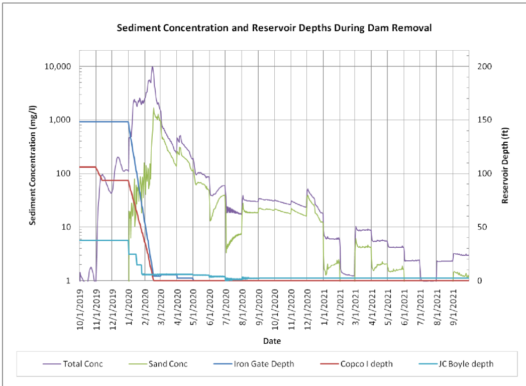
Figure 5.15. Reservoir depth and sediment concentrations downstream of Iron Gate Dam during drawdown for a median year.
