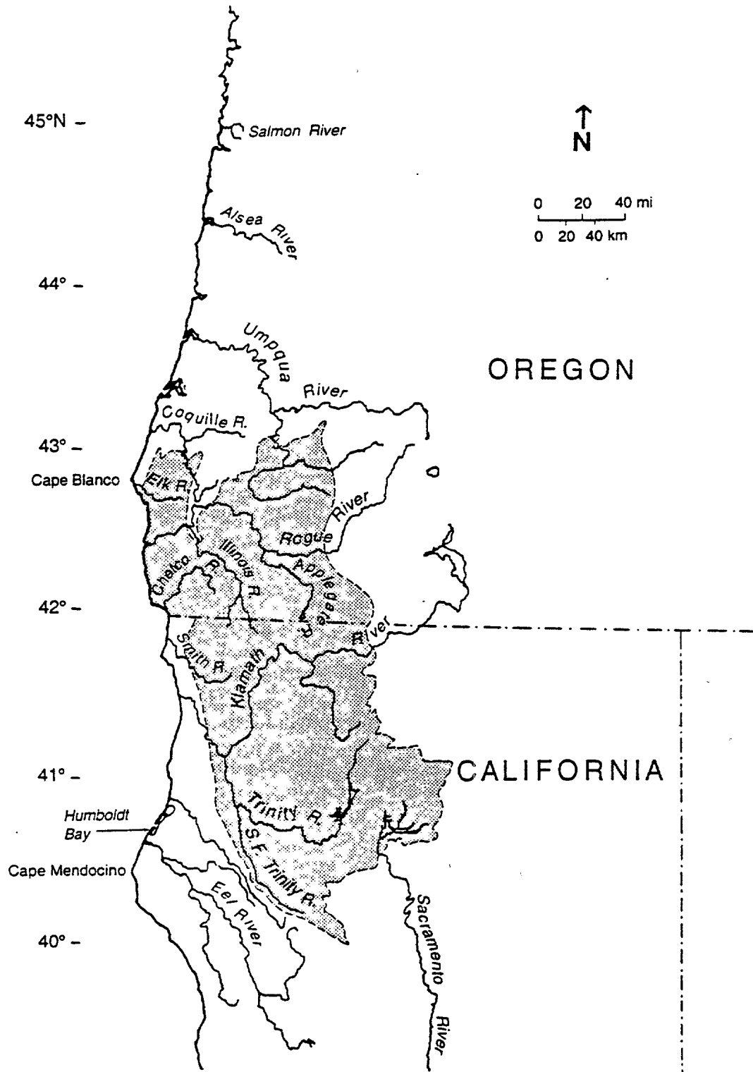
Figure 2. Map of the southern Oregon-northern California area. Shaded area is the Klamath Mountains Geologic Province (modified from Irwin 1966 and Walker and MacLeod 1991).
