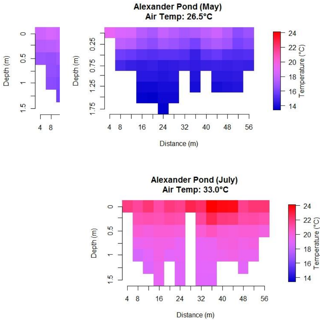
Figure 10. Alexander Pond temperature stratification May through July, 2014. Data collected from multiple depths along the pond centerline every four meters. (Krall, raw data, 2014).
