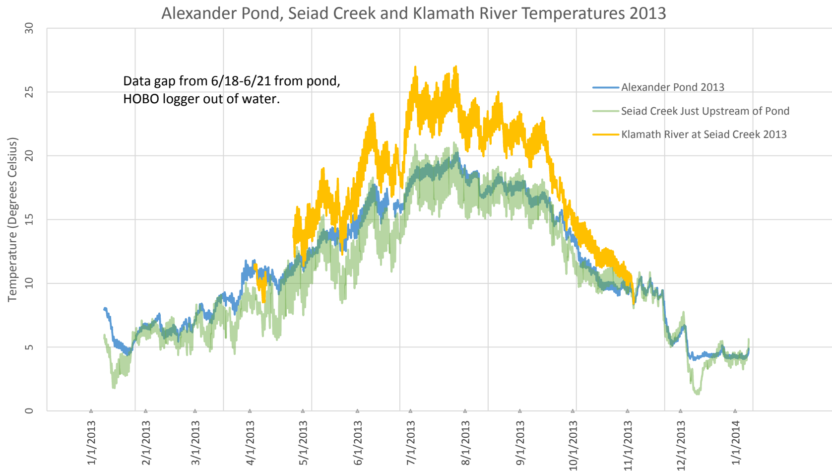
Figure 8. Alexander Pond and Seiad Creek temperatures from HOBO loggers and Klamath River temperatures from the Karuk Water Quality Program's DataSonde for 2013. Grapho shows Alexander Pond provides suitable thermal refuge for rearing coho salmon year round, and less diel variation and higher winter temperatures than adjacent Seiad Creek.
