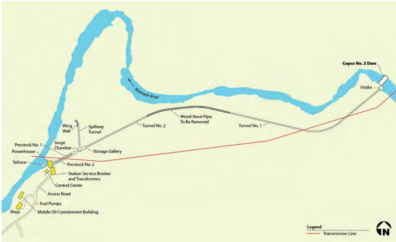
Figure 4.2-13: Map of the Copco 2 Dam and Associated Facilities.
